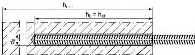
Reinforcing bar
