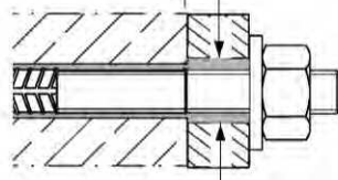
UPAT rebar anchor Push through anchor (annular gap filled with mortar)
